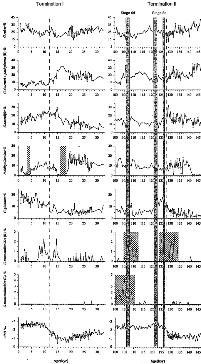
Figure 3. The variations of relative abundances of five dominant planktic foraminifer species and two deep-dwelling species against age of the last two Terminations in MD972151. The planktic foraminifer \delta^{18}\text{O} data from the same core are plotted for comparison and age model construction. The two Termination boundaries are indicated by dashed lines. Hatched shadows indicate events of Pulleniatina minima in the Holocene (Ujiié and Ujiié, 1999) and increased abundances of deep-dwelling species G. truncatulinoides (left coiling) and G. truncatulinoides (right coiling) in stage 5d and 5e (Jian et al., 2000). The shaded lines indicate dust peak events in stage 5d and 5e reported from loess profiles in central China (An and Porter, 1997).
