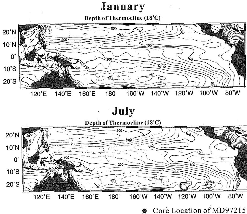
Figure 2. Modern January and July distributions of depth of thermocline (DOT) in the tropical Pacific (modified from Andreasen and Ravelo, 1997). Shallow DOTs are found from the eastern and deep DOTs are from the western Pacific. The dot indicates the location of IMAGES core MD972151.
