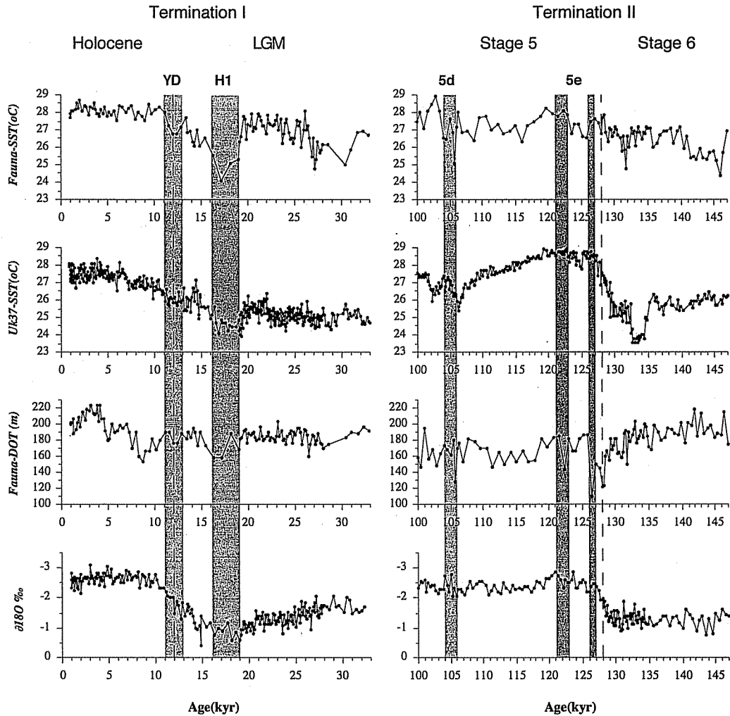
Figure 5. Variations of faunal estimates sea-surface temperature (SST), depth of thermocline (DOT), and U^{37} plotted against age during the last two Terminations. The SST estimates were computed based on a global transfer function (Ortiz and Mix, 1997), and the DOT estimates were based on a tropical Pacific Ocean transfer function (Andreasen and Ravelo, 1997). Termination boundaries are indicated by dashed vertical lines. The shaded lines indicate intervals of the Younger Dryas and Heinrich events (in left panel) and dust peak events in stage 5d and 5e reported from loess profiles in central China (An and Porter, 1997).
