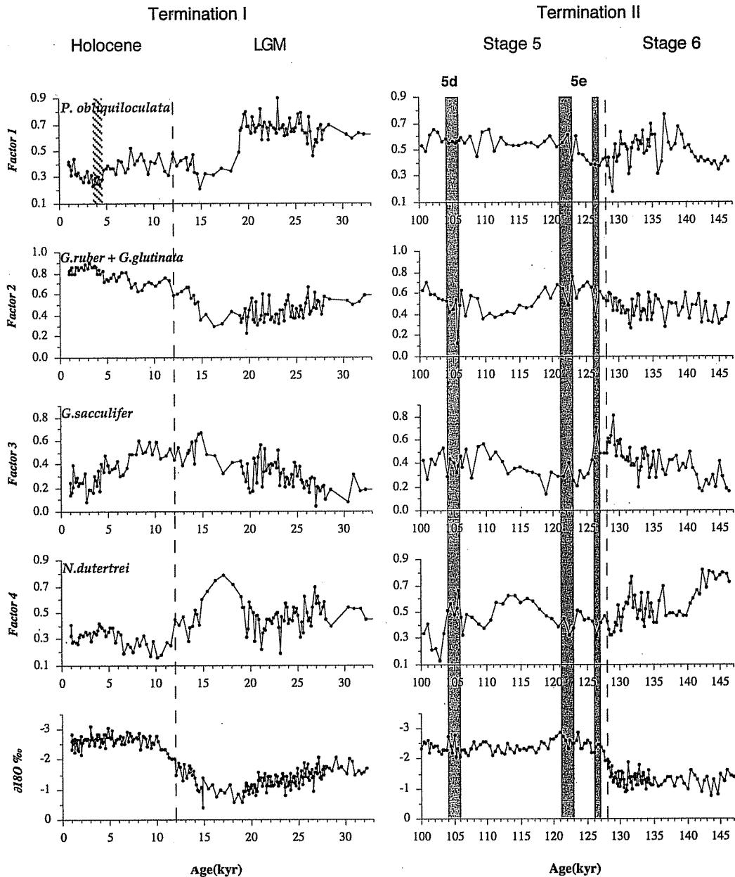
Figure 4. The variations of four important faunal factors from core MD972151 of the last two Terminations and of planktic foraminifer G. sacculifer \delta^{18}O plotted against age. The factors were computed using a Q-mode factor analysis with a VARIMAX solution (Klovan and Imbrie, 1971). Termination boundaries are indicated by dashed vertical lines. The shaded lines indicate intervals of the Younger Dryas and Heinrich events (in left panel) and dust peak events in stage 5d and 5e reported from loess profiles in central China (An and Porter, 1997).
